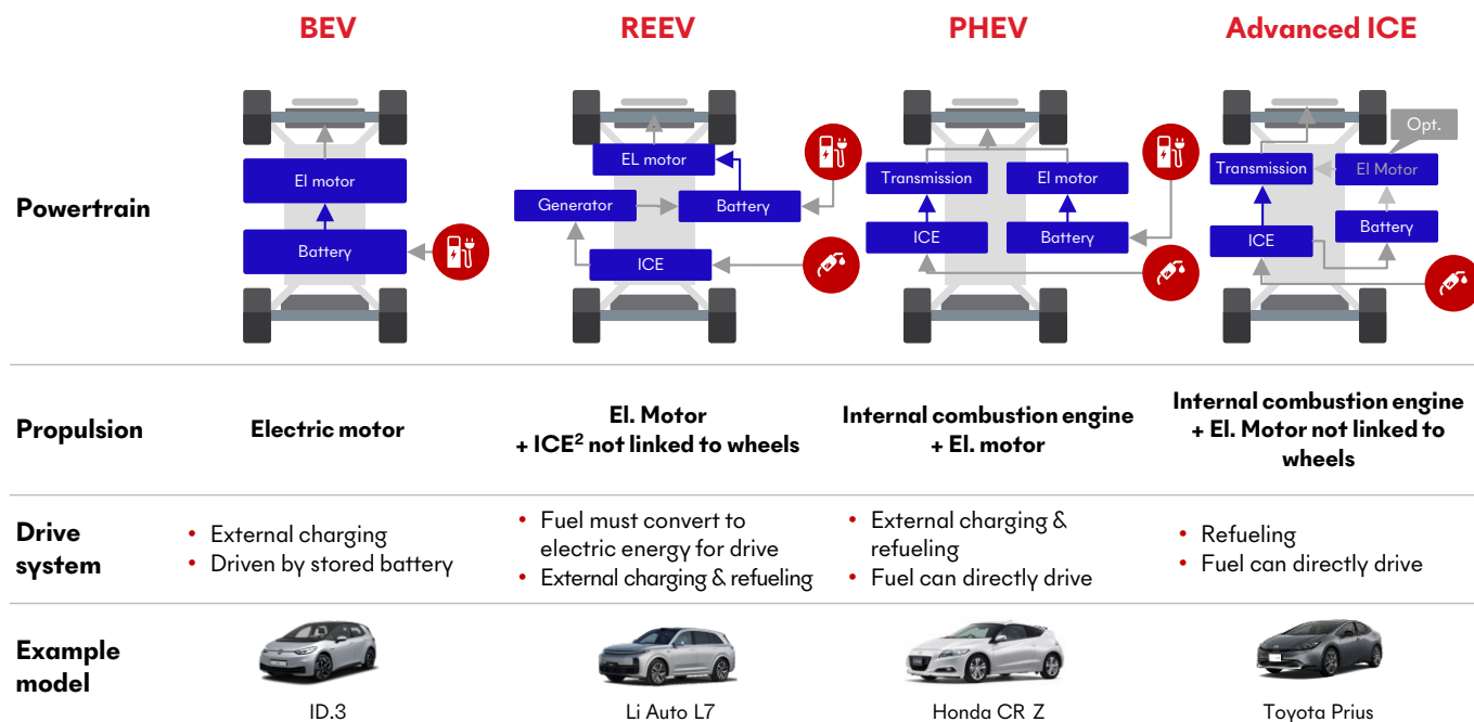
FIGURE 2: POWERTRAIN CATEGORIES
