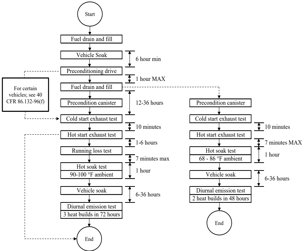
Figure 1 to paragraph (e) of § 1066.801—FTP Test Sequence
