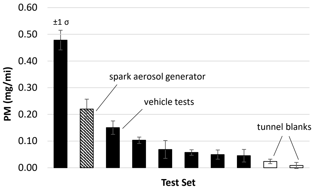
Figure 16: Example of test-to-test repeatability of PM measurements from vehicles without and with GPF, an aerosol generator, and tunnel blanks from two EPA test cells.
