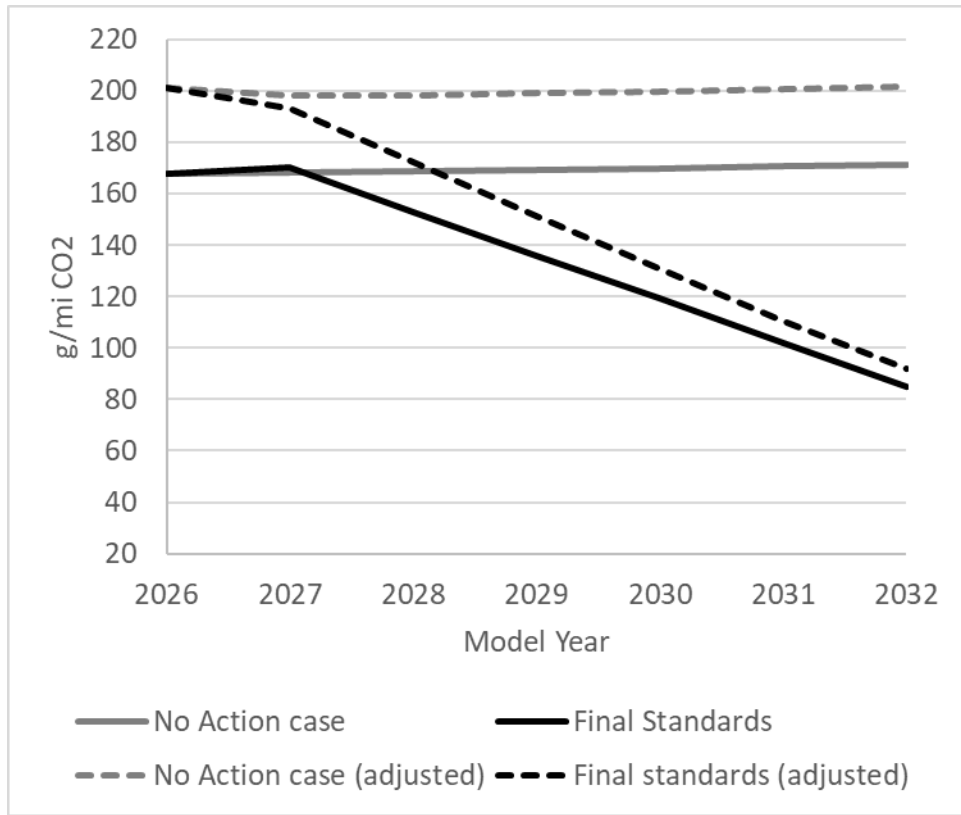
Figure 9: Projected industry average targets under the final 2027-2032 standards compared to the current MY 2026 standards. Adjusted targets include effects of projected off-cycle, A/C efficiency and A/C leakage credits.
