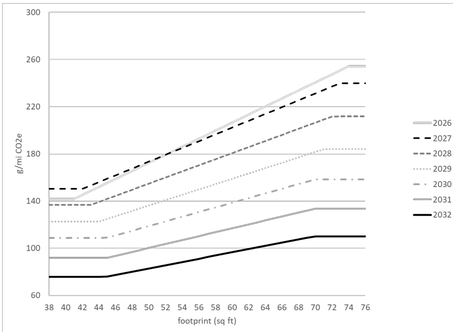
Figure 8: Final standards for trucks, MY 2027-2032.
