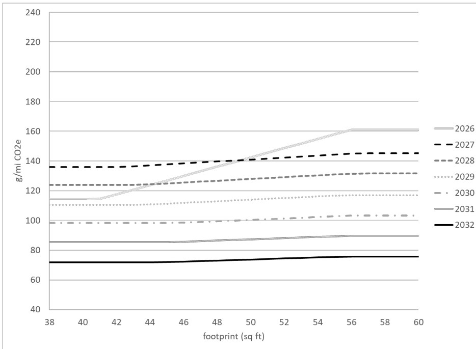
Figure 7: Final standards for cars, MY 2027-2032.
