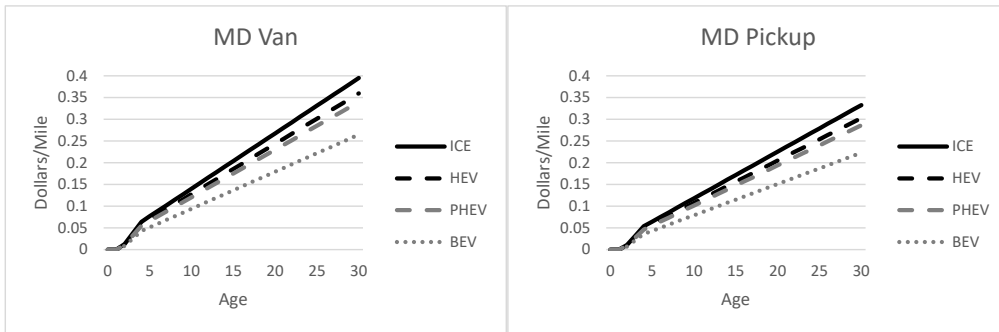
Figure 46: Repair cost per mile (2019 dollars) for a $35,000 medium-duty van and pickup with various powertrains by vehicle age in years.
