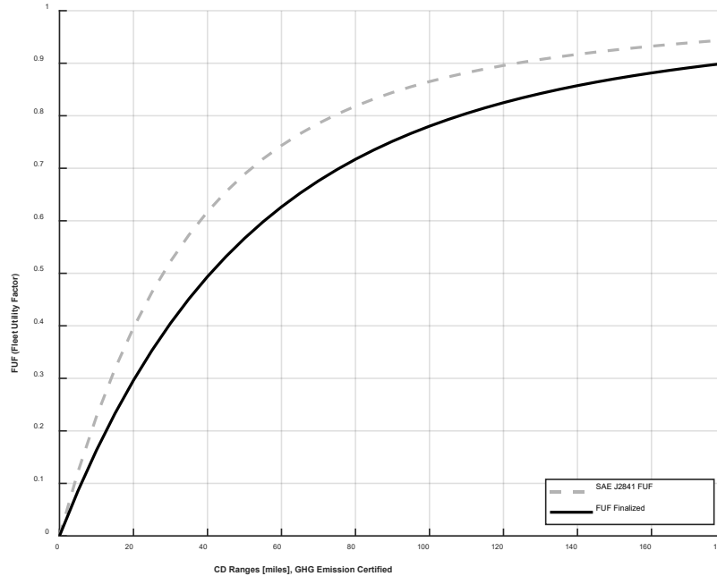
Figure 11: SAE J2841 FUF and finalized FUF (Fleet Utility Factor) for PHEV compliance.
