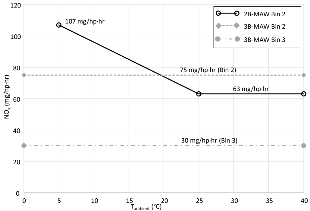
Figure 18: 2B-MAW bin 2 in-use NO x standard with ambient temperature correction and PEMS accuracy margin compared to 3B-MAW bin 2 and bin 3 in-use NO x standard.
