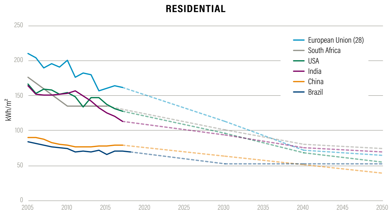
Figure 27 | Historical trends and required declines in the energy intensity of residential buildings
