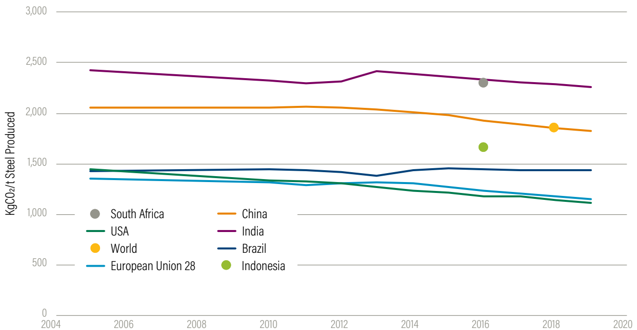
Figure 32 | Carbon intensity of steel production, 2005–19
