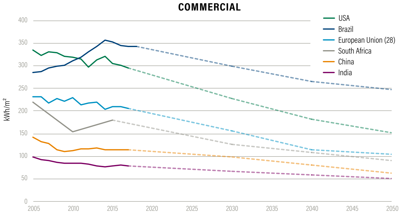
Figure 28 | Historic trends and required declines in the energy intensity of commercial buildings
