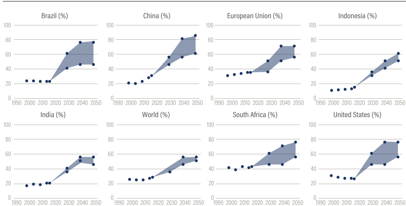
Figure 34 | Share of electricity in industrial energy use (%)
