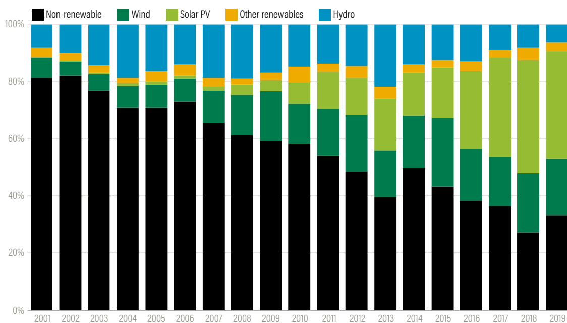
Figure 16 | Growing share of renewables in annual additions to global installed generating capacity, 2001–19
