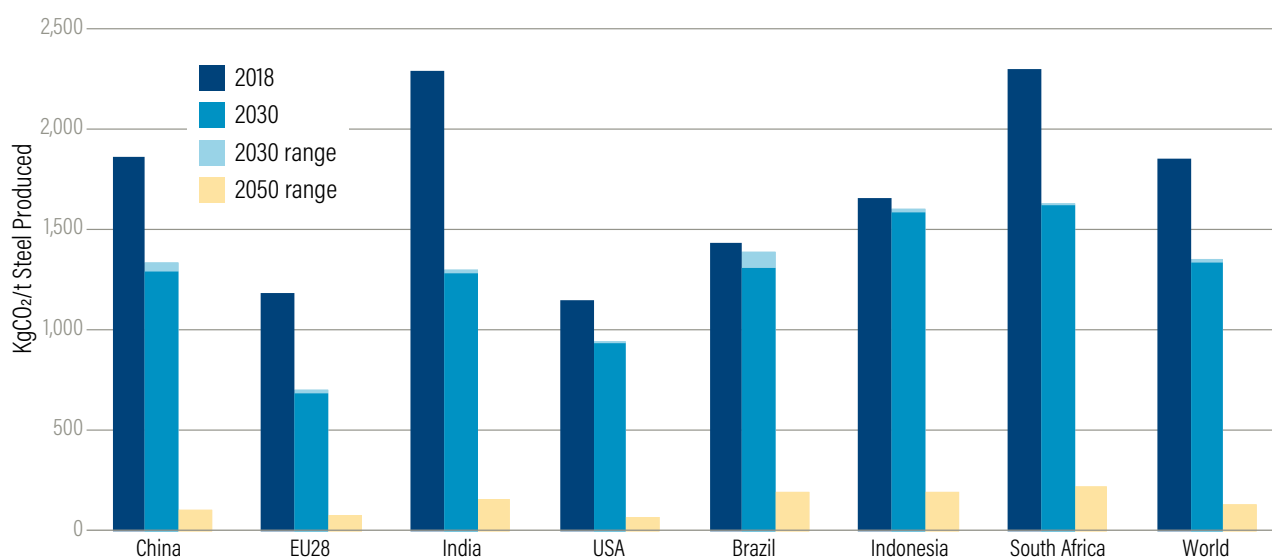
Figure 33 | Carbon intensity of steel production in 2018 and targets for 2030 and 2050
