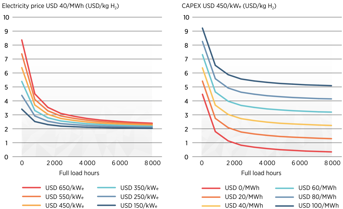
Figure 4.3. Future levelised cost of hydrogen production by operating hour for different electrolyser investment (left) and electricity costs (right)
