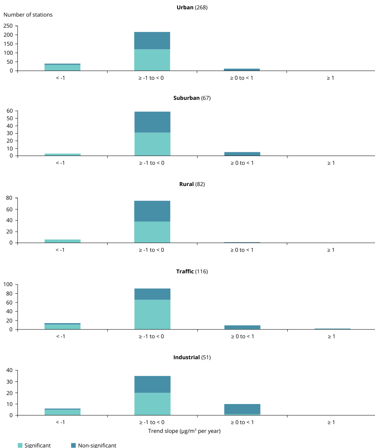
Figure 4.9 Trend slope distribution (2009-2018) for PM 2.5 annual mean concentration, per station type, for both significant and non-significant trends
