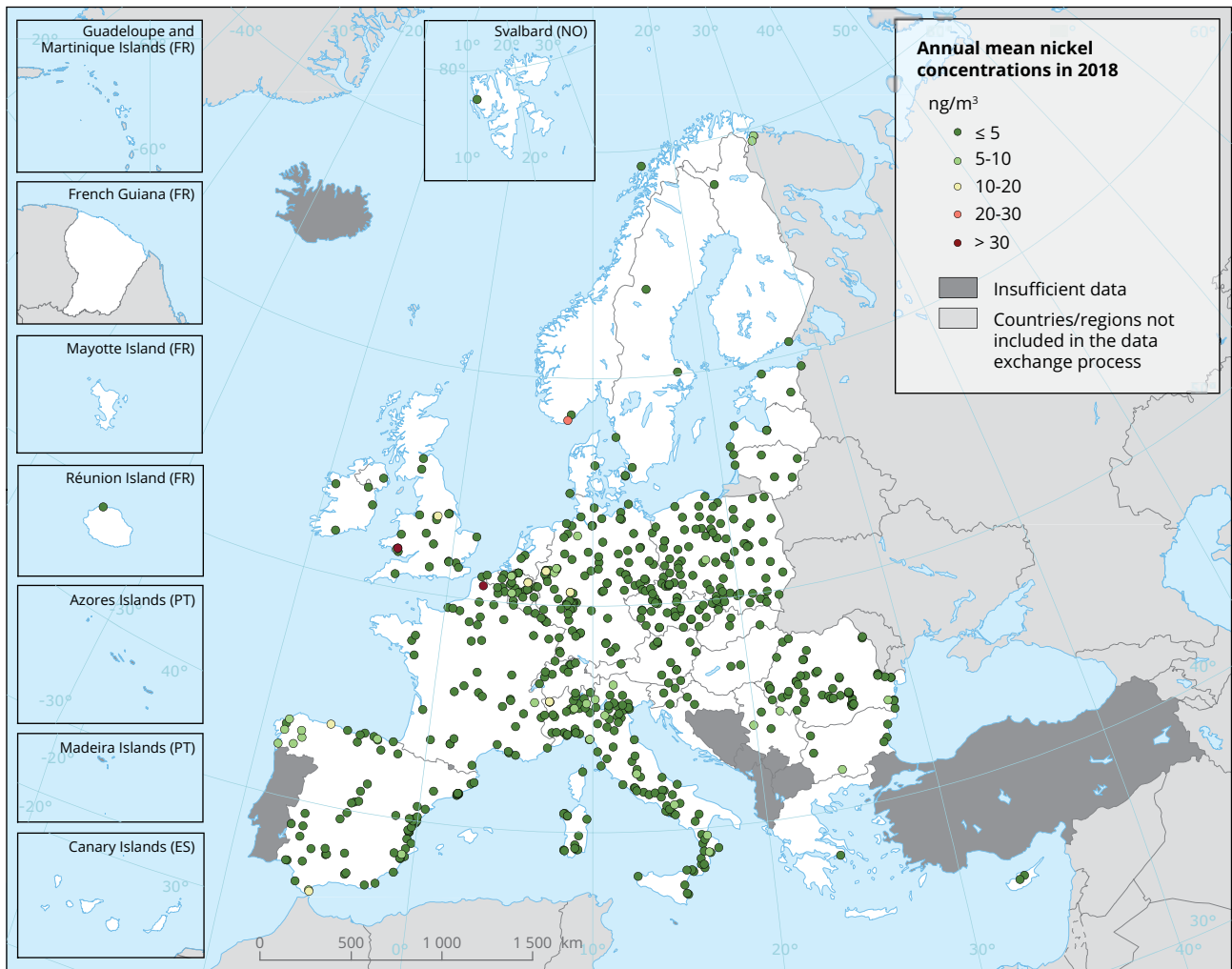
Map 8.7 Concentrations of Ni, 2018
