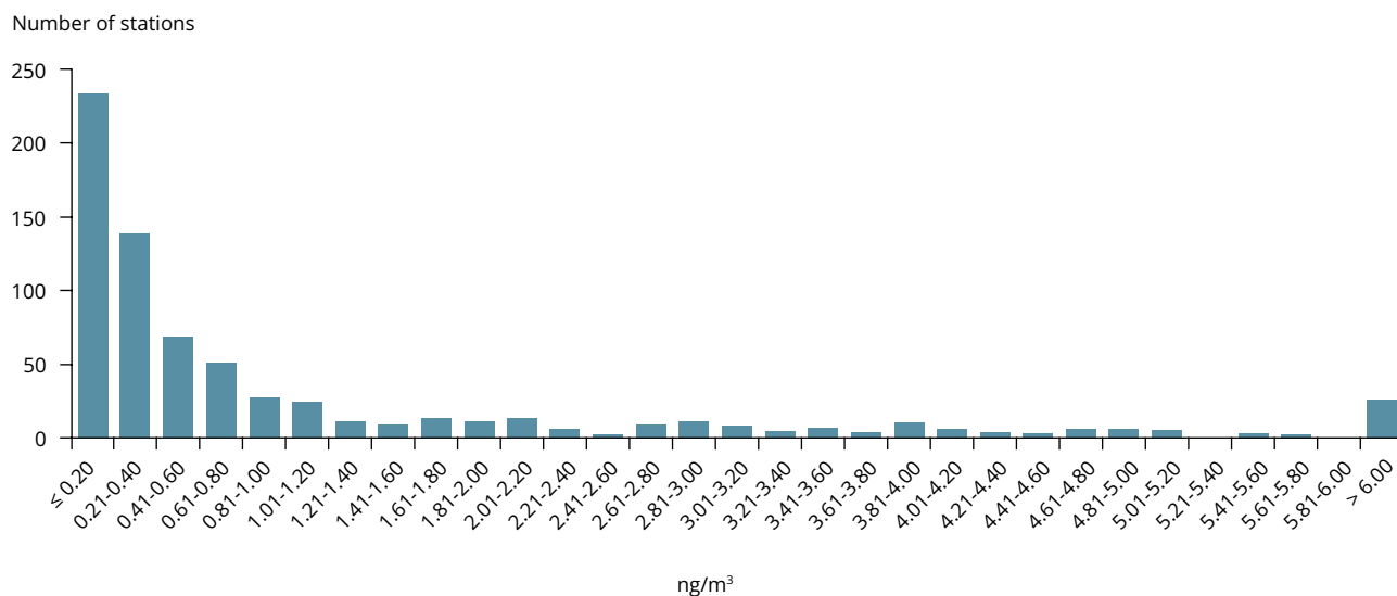
Figure A1.12 Annual mean concentrations of BaP by station and area type, 2018
