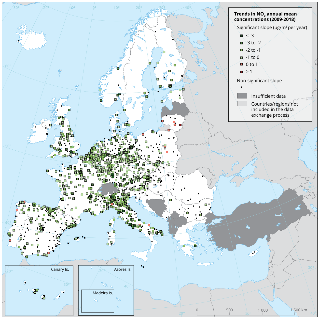
Map 6.2 Trends in NO 2 annual mean concentrations (2009-2018)
