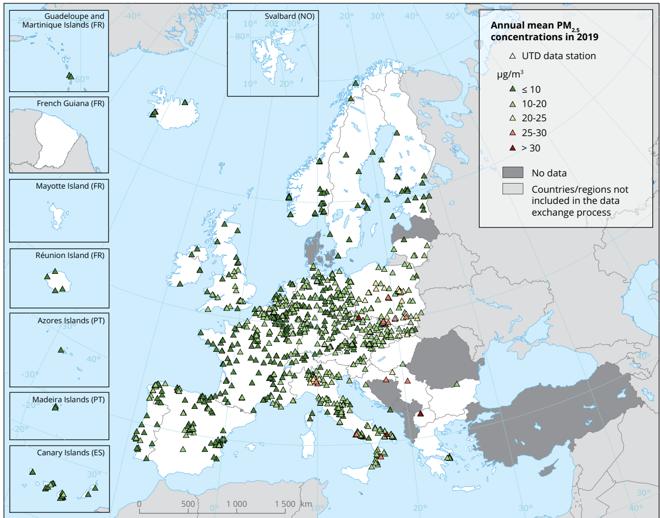
Map 4.8 Concentrations of PM 2.5 , 2019 — annual limit value
