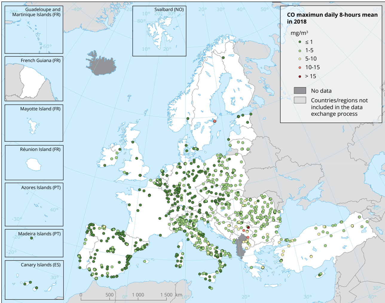
Map 8.2 Concentrations of CO, 2018
