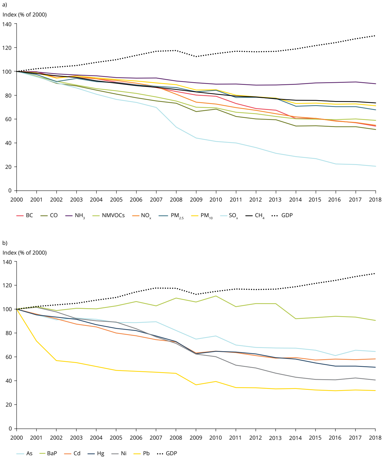
Figure 3.1 Development in EU-28 emissions, 2000-2018 (% of 2000 levels): (a) SO x , NO x , NH 3 , PM 10 , PM 2.5 , NMVOCs, CO, CH 4 and BC; (b) As, Cd, Ni, Pb, Hg and BaP. Also shown for comparison is the EU-28 GDP (expressed in chain-linked volumes (2010), % of 2000 level)
