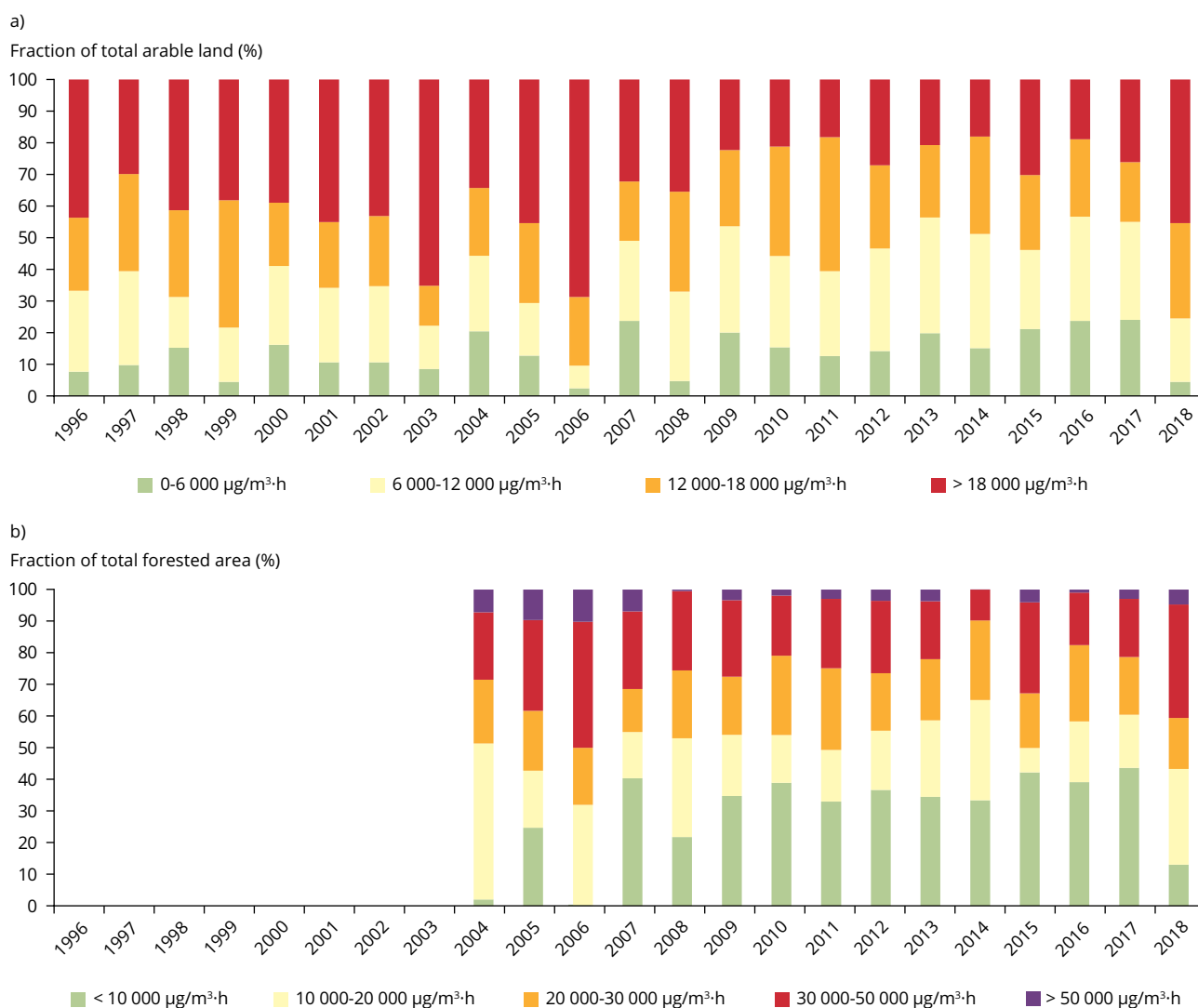
Figure 11.1 Exposure of (a) agricultural area and (b) forest area to O 3 (AOT40) in the EEA member countries, from 1996 (a) and 2004 (b) to 2018
