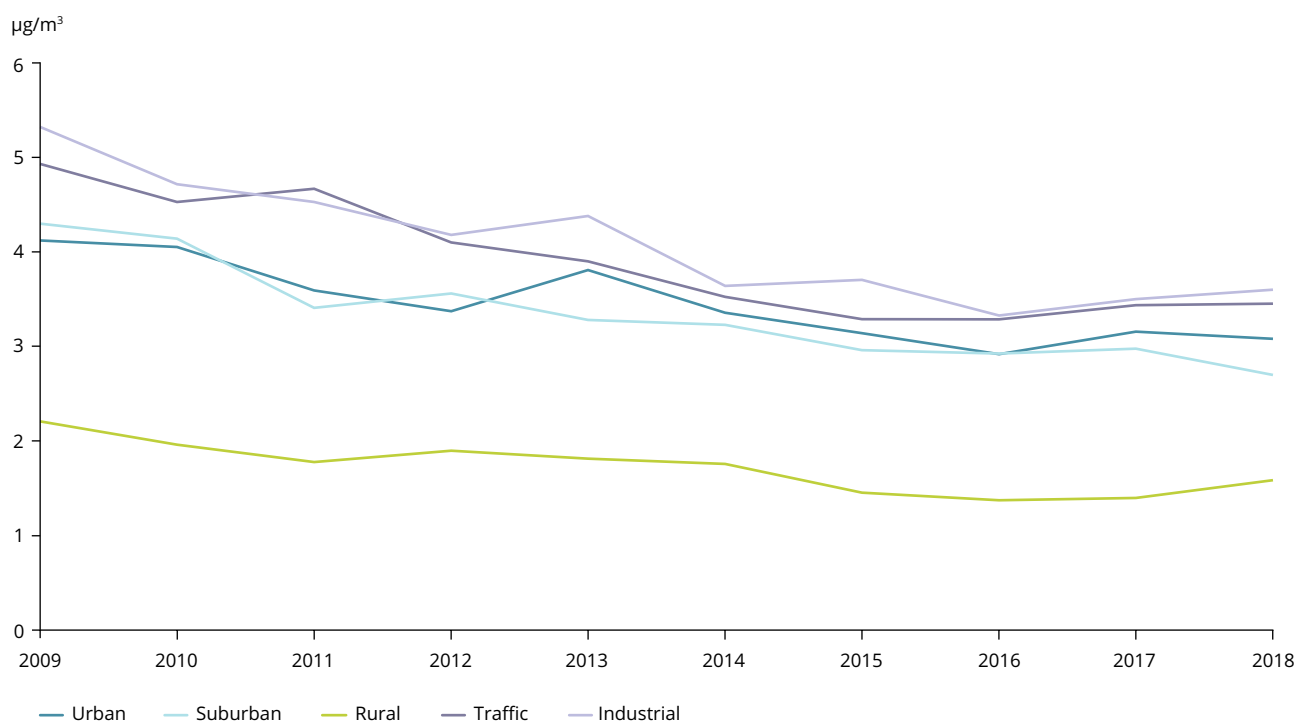
Figure 8.1 Average SO 2 annual mean concentrations by station type
