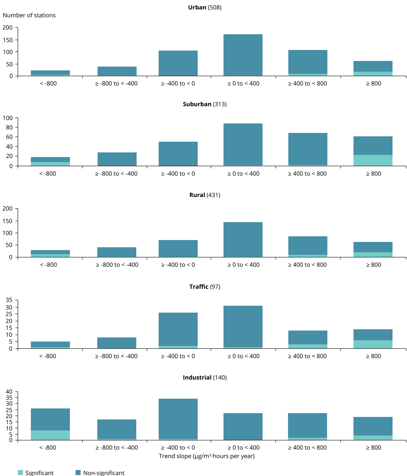
Figure 11.3 Trend slope distribution (2009-2018) for O 3 indicator AOT40 for vegetation and crops, per station type, for both significant and non-significant trends
