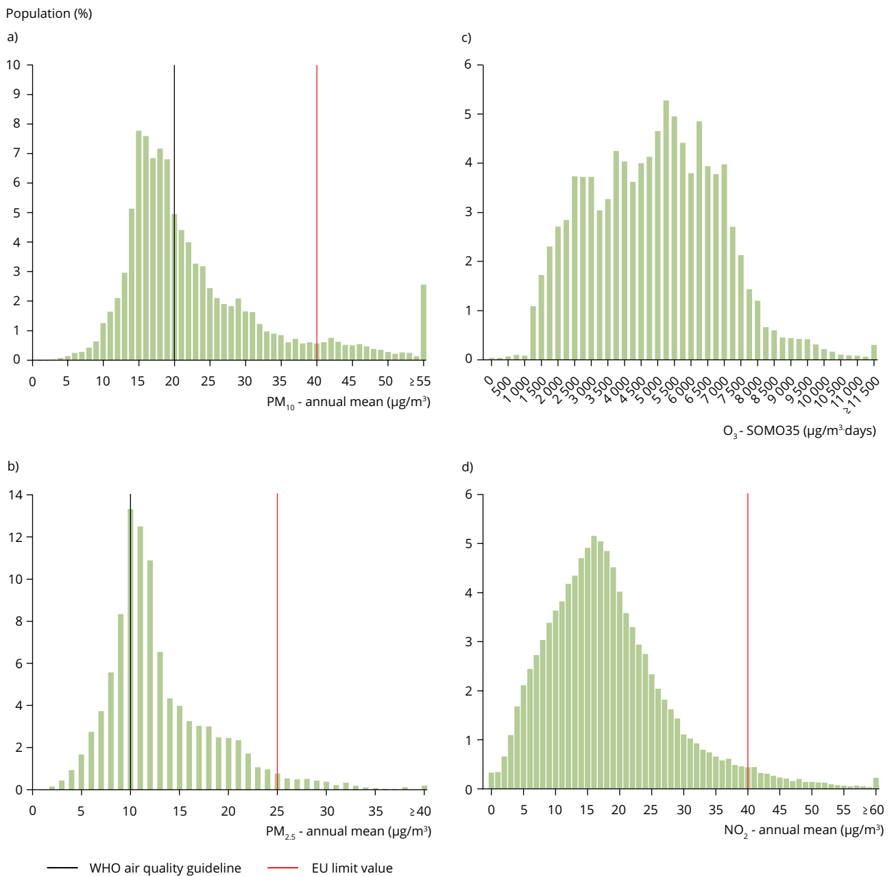
Figure 9.1 Frequency distribution of the total population exposure to PM 10 (annual mean), PM 2.5 (annual mean), O 3 (SOMO35) and NO 2 (annual mean) in 2018
