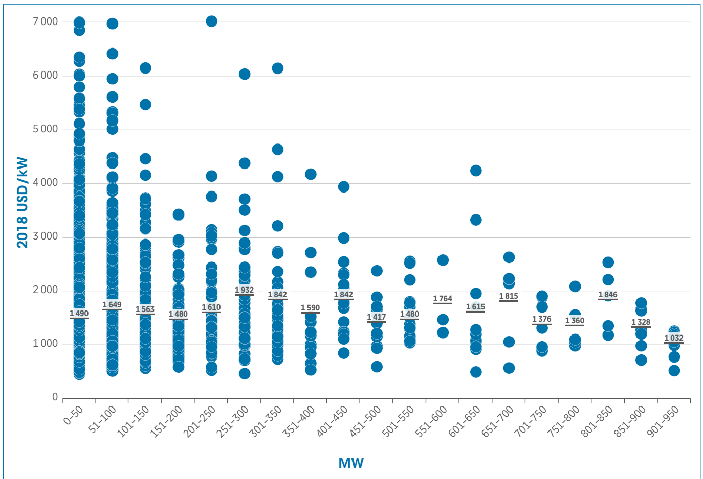
Figure 5.2 Total installed costs for hydropower by project and weighted average by capacity range, 2000–2018
