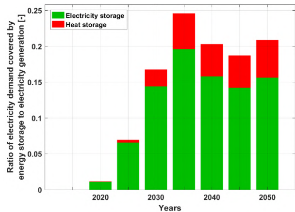
Figure 3.5-4: Sub-Saharan Africa – Electricity demand covered by energy storage (left) and ratio of electricity demand covered by different forms of energy storage (right) during the energy transition from 2015 to 2050.
