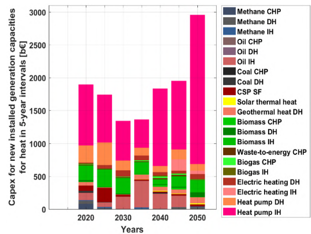
Figure 3.1-13: Global – Capital costs of installed generation capacities in five-year intervals for electricity (left) and heat (right) during the energy transition from 2015 to 2050.
