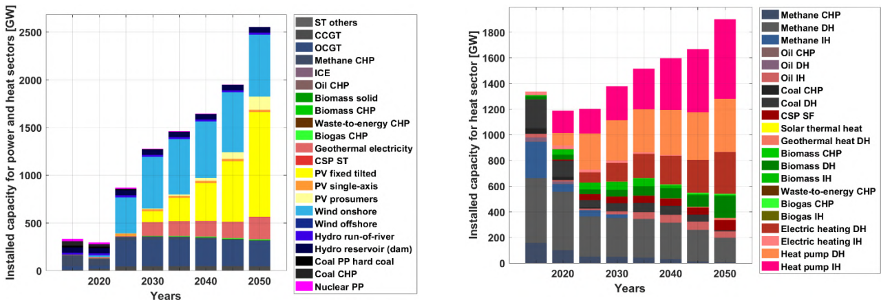
Figure 3.3-8: Technology-wise installed capacities for power (left) and heat (right) during the energy transition from 2015 to 2050 in Europe.
