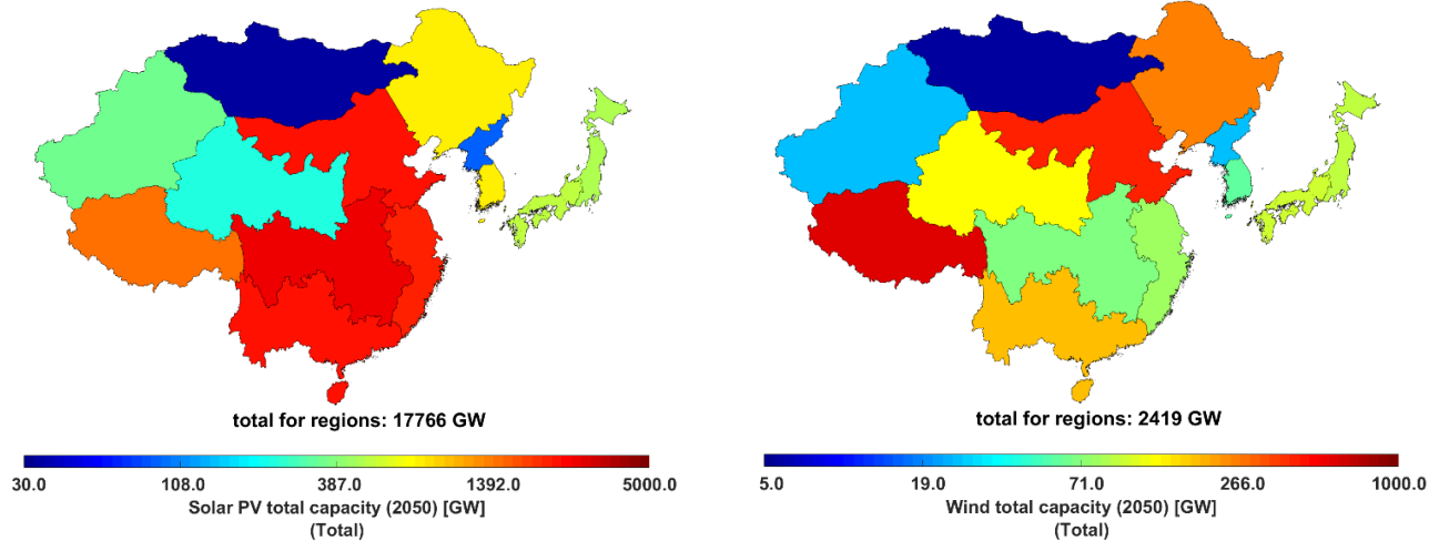
Figure 3.7-26: Northeast Asia – Regional variation of electricity generation capacities of solar PV (left) and wind energy (right) in 2050.
