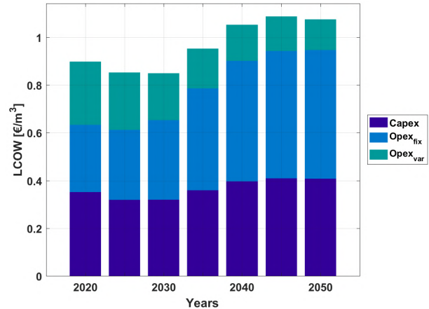
Figure 3.10-24: South America – Capital costs for five-year intervals (left) and levelised cost of water (right) during the energy transition from 2015 to 2050.
