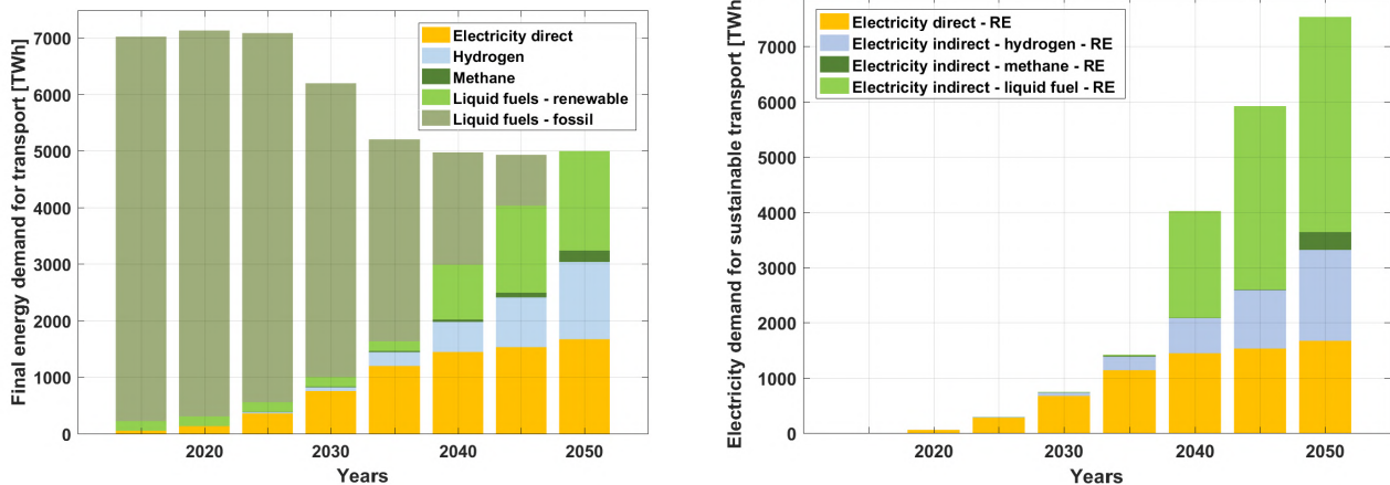
Figure 3.2-14: Europe – Final energy demand for transport (left) and electricity demand for sustainable transport (right) during the energy transition from 2015 to 2050.
