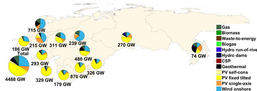
Figure 3.3-25: Eurasia – Regional electricity generation capacities (top) and electricity generation (bottom) in 2050.
