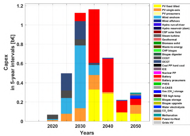
Figure 3.5-24: Sub-Saharan Africa – Capital costs for five-year intervals (left) and levelised cost of water (right) during the energy transition from 2015 to 2050.
