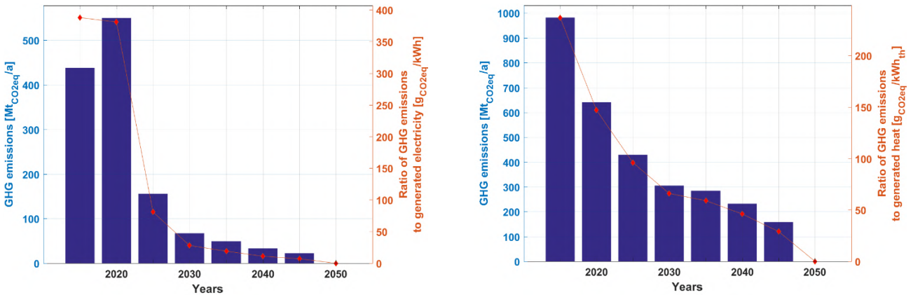
Figure 3.3-31: Eurasia – GHG emissions in the power sector (left) and GHG emissions in the heat sector (right) during the energy transition from 2015 to 2050.
