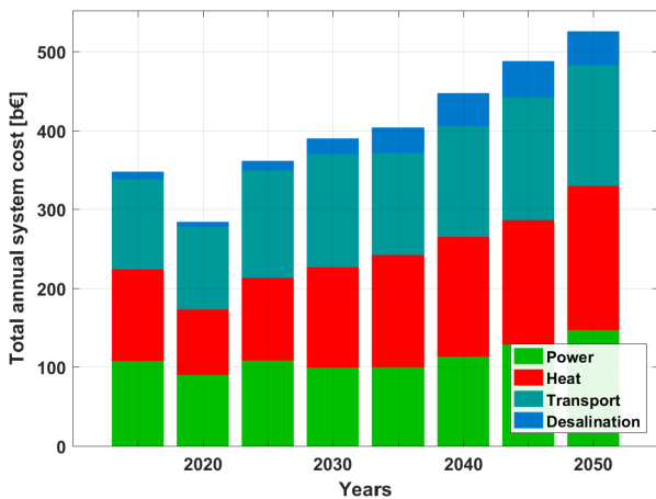
Figure 3.4-6: MENA – Annual system costs, sector-wise (left) and functionality-wise (right) during the energy transition from 2015 to 2050.
