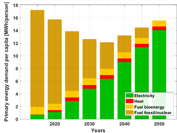
Figure 3.1-1: Global – Primary energy demand sector-wise (top left), efficiency gain in primary energy demand (top right), electricity consumption per capita with population (bottom left) and primary energy demand per capita (bottom right) during the energy transition from 2015 to 2050.
