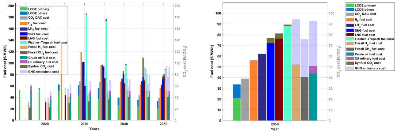
Figure 3.3-19: Eurasia – Fuel costs for the transport sector during the energy transition from 2015 to 2050 (left) and fuel costs in 2050 (right).
