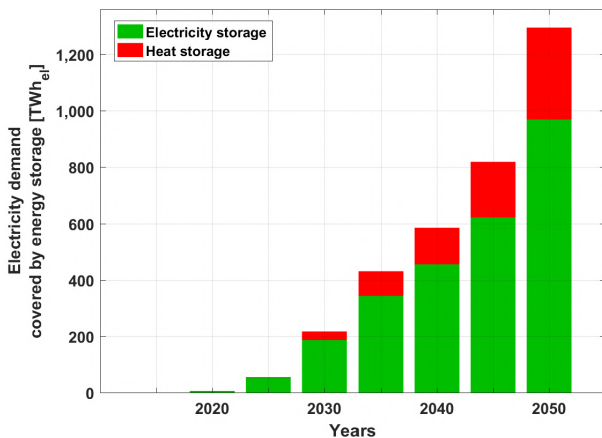
Figure 3.5-4: Sub-Saharan Africa – Electricity demand covered by energy storage (left) and ratio of electricity demand covered by different forms of energy storage (right) during the energy transition from 2015 to 2050.
