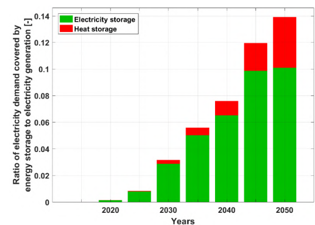
Figure 3.3-4: Eurasia – Electricity demand covered by energy storage (left) and ratio of electricity demand covered by different forms of energy storage (right) during the energy transition from 2015 to 2050.
