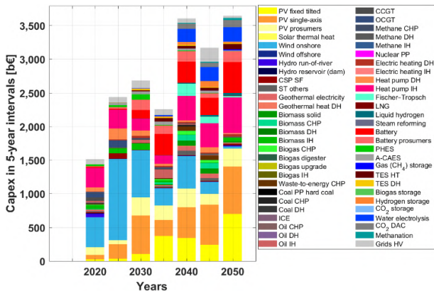
Figure 3.7-7: Northeast Asia – Capital costs for five-year intervals (left) and levelised cost of energy (right) during the energy transition from 2015 to 2050.
