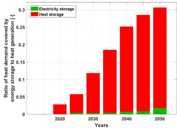
Figure 3.4-5: MENA – Heat demand covered by energy storage (left) and the ratio of heat demand covered by different forms of energy storage (right) during the energy transition from 2015 to 2050.
