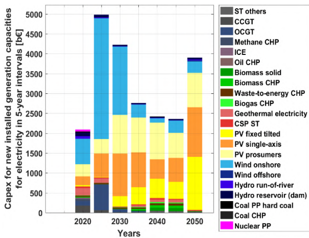
Figure 3.1-13: Global – Capital costs of installed generation capacities in five-year intervals for electricity (left) and heat (right) during the energy transition from 2015 to 2050.
