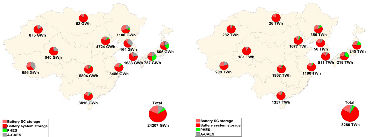
Figure 3.7-28: Northeast Asia – Regional electricity storage capacities (left) and electricity storage annual throughput (right) in 2050.
