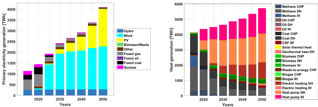
Figure 3.3-9: Eurasia – Primary electricity generation (left) and technology-wise heat generation (right) during the energy transition from 2015 to 2050.
