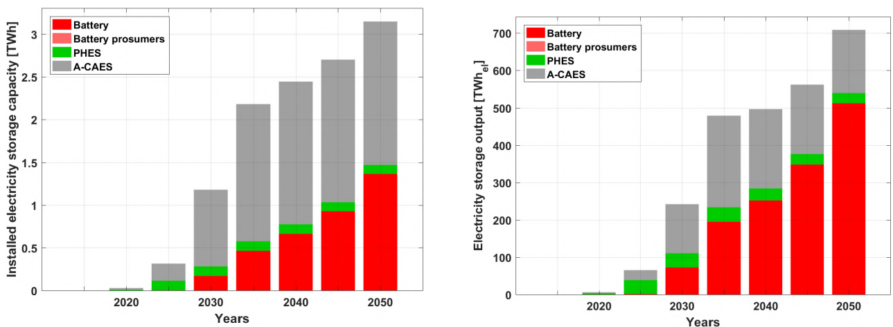
Figure 3.2-16: Europe – Transport sector installed electricity storage capacity (left) and electricity storage output (right) during the energy transition from 2015 to 2050.
