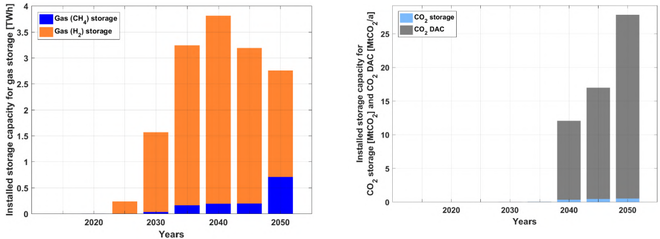
Figure 3.3-18: Eurasia – Transport sector installed capacity for gas (methane and hydrogen) storage (left) and CO 2 direct air capture and CO 2 storage (right) during the energy transition from 2015 to 2050.
