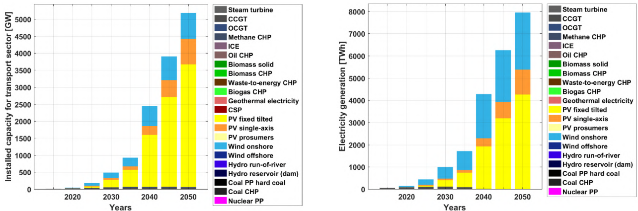
Figure 3.2-15: Europe – Transport sector installed power generation capacity (left) and electricity generation (right) during the energy transition from 2015 to 2050.
