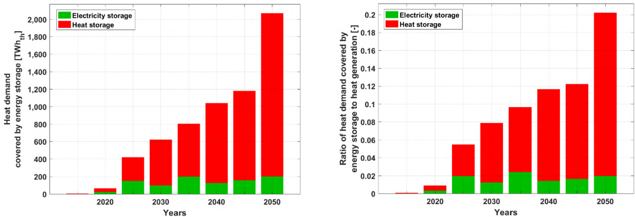
Figure 3.2-5: Europe – Heat demand covered by energy storage (left) and the ratio of heat demand covered by different forms of energy storage (right) during the energy transition from 2015 to 2050.
