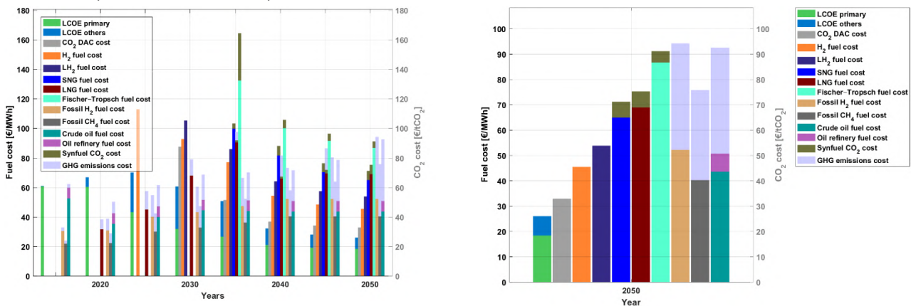
Figure 3.4-19: MENA – Fuel costs for the transport sector during the energy transition from 2015 to 2050 (left) and fuel costs in 2050 (right).
