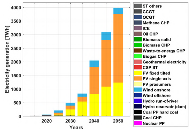
Figure 3.4-15: MENA – Transport sector installed power generation capacity (left) and electricity generation (right) during the energy transition from 2015 to 2050.
