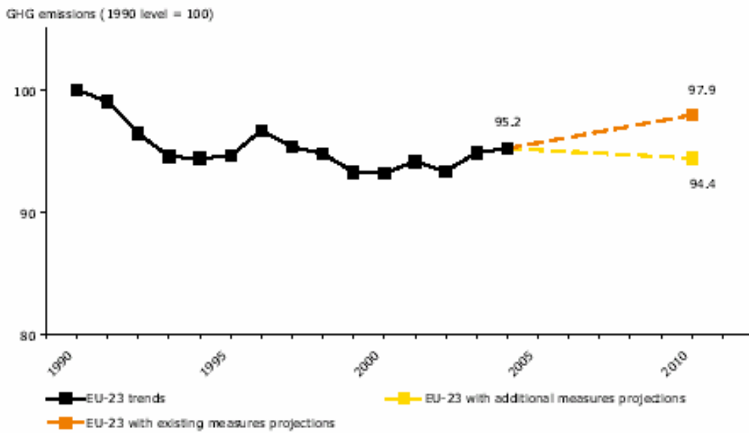
Figure 3.1 Greenhouse gas emission trends and projections for EU-23
